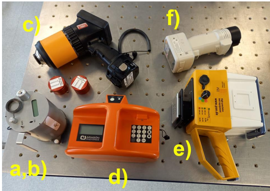
Figure 1. Handheld reflectometer models: a) 15R(-USB) (similar design as b) 15R-RGB) by D&S, c) 410-Solar by SOC, d) Condor by Aragon Photonics, e) pFlex by PSE, f) CM-700d by Konica Minolta.
