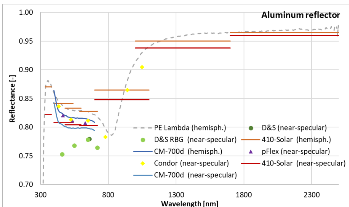
Figure 5. Reflectance spectra of aluminum mirror measured with all devices.
