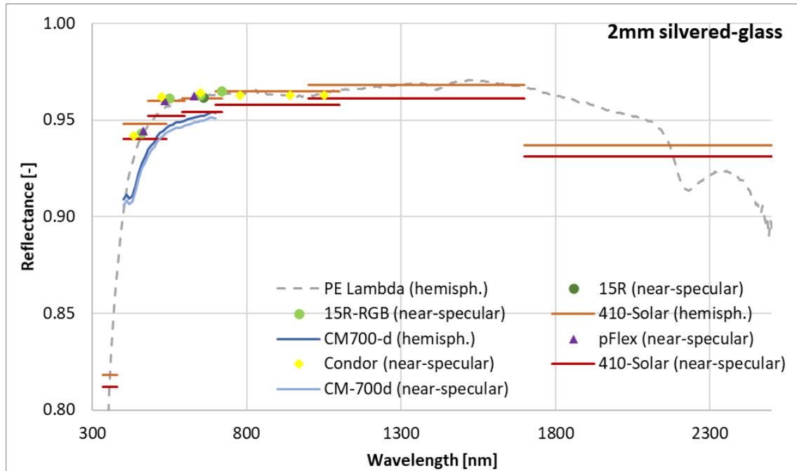
Figure 2. Reflectance (hemispherical and near-specular) spectra of a clean and non-degraded 2 mm silvered-glass mirror measured with all devices.
