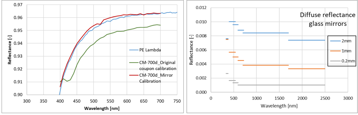
Figure 3. left: Comparison of measurements with different calibration coupons for the CM-700d, right: diffuse reflectance measured of mirrors with different glass thickness with 410-Solar.
